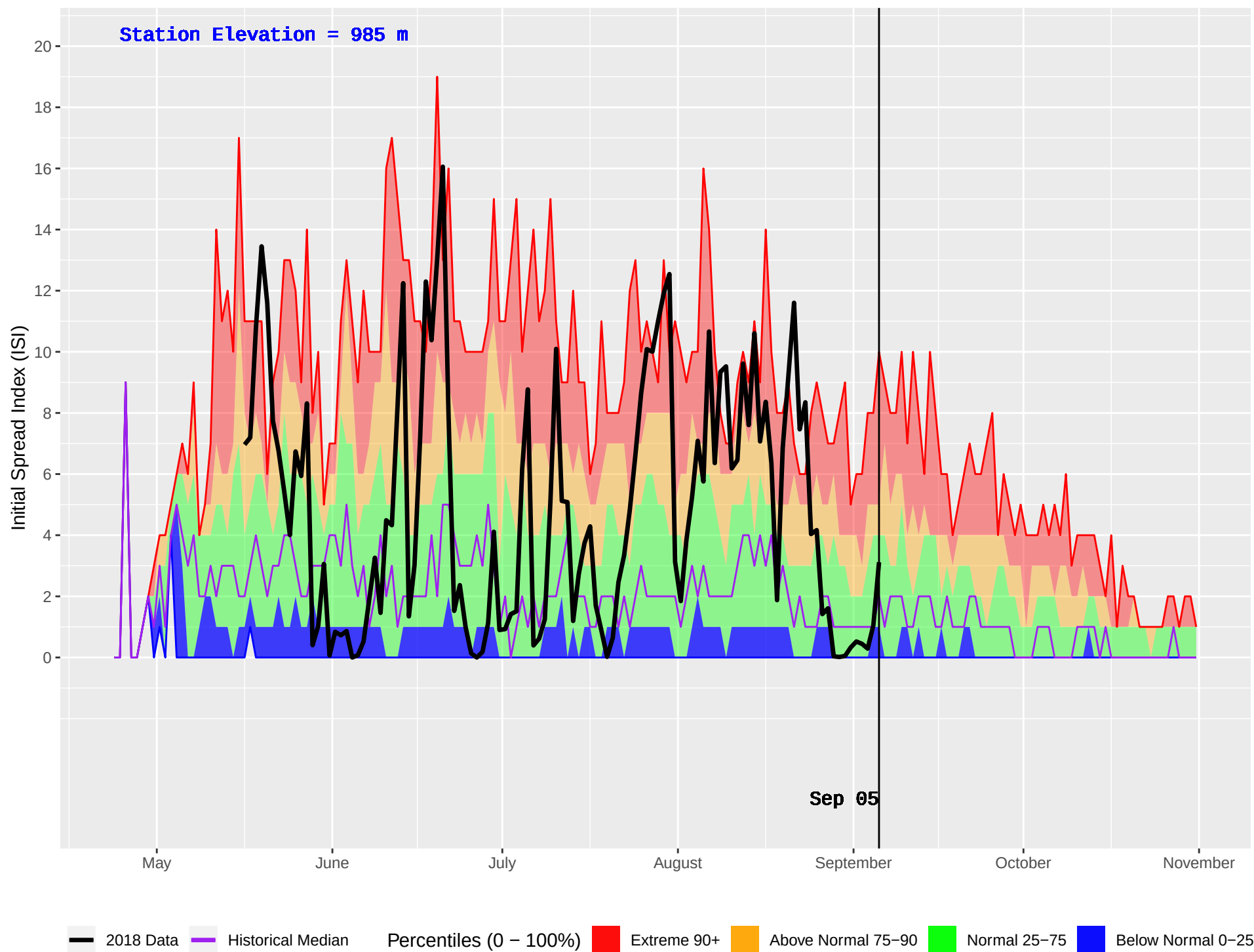
SIFTON (152) : Historical (1988–2016) and Current (2018) Daily Initial Spread Index (ISI)
