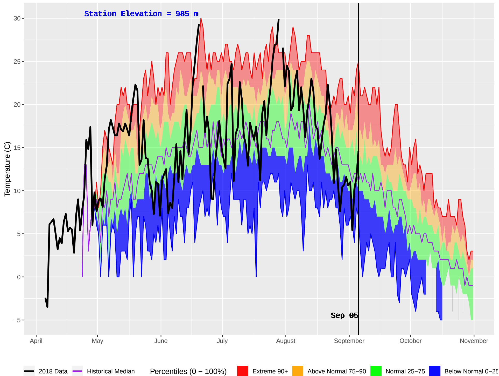
SIFTON (152) : Historical (1988–2016) and Current (2018) Daily Temperature
