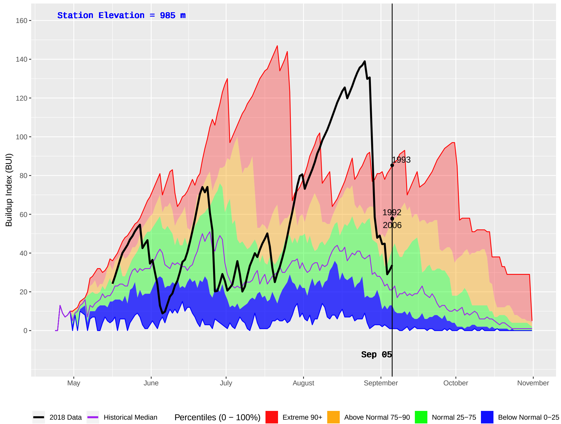
SIFTON (152) : Historical (1988–2016) and Current (2018) Daily Buildup Index (BUI)
