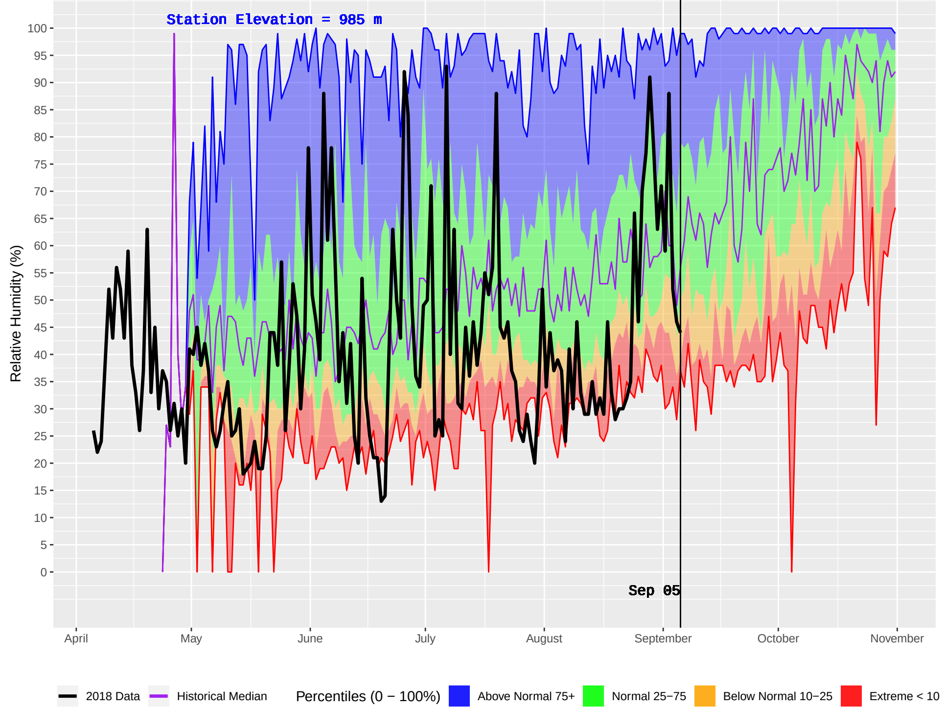
SIFTON (152) : Historical (1988–2016) and Current (2018) Daily Relative Humidity
