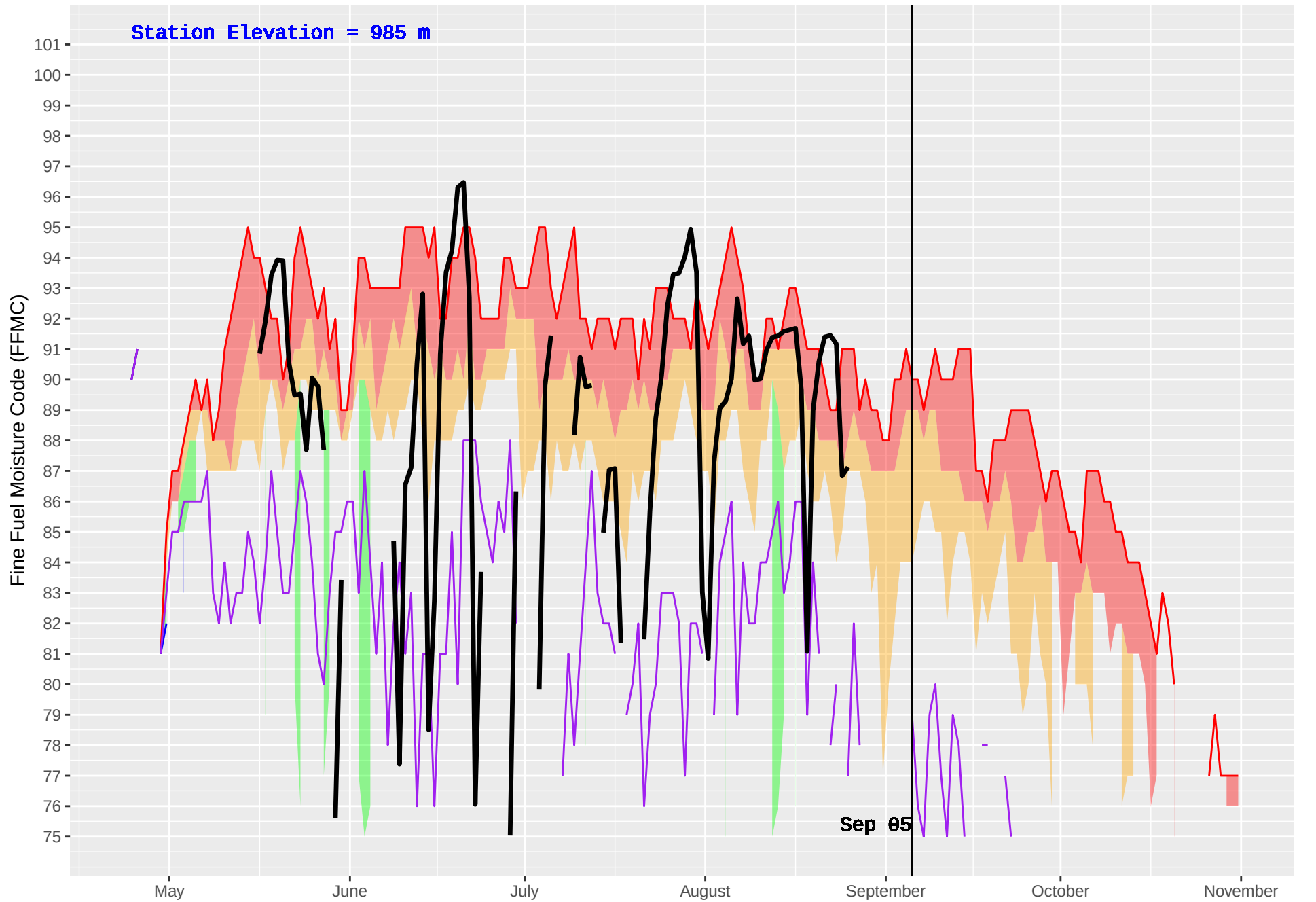
SIFTON (152) : Historical (1988–2016) and Current (2018) Daily Fine Fuel Moisture Code (FFMC)
