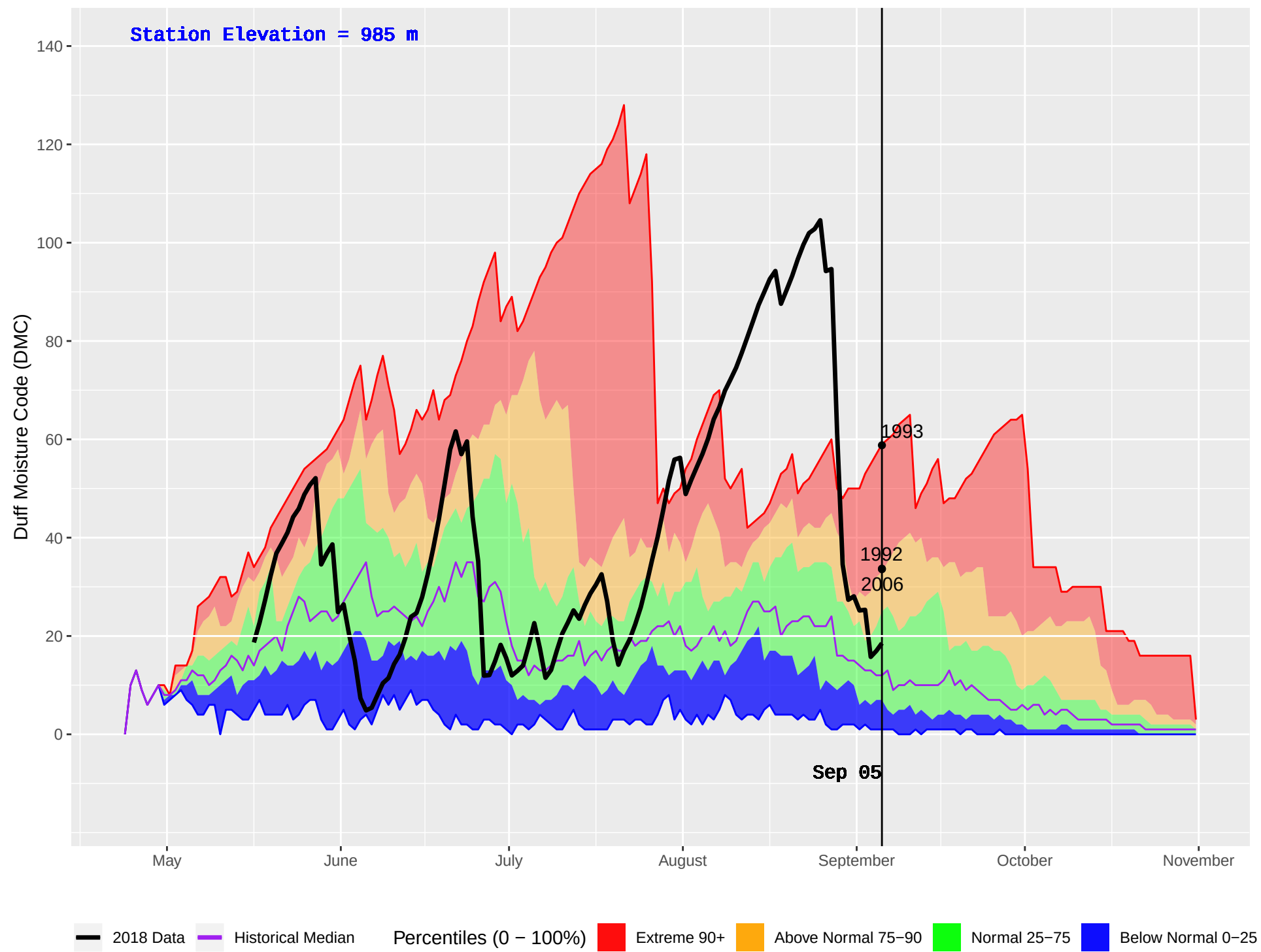
SIFTON (152) : Historical (1988–2016) and Current (2018) Daily Duff Moisture Code (DMC)
