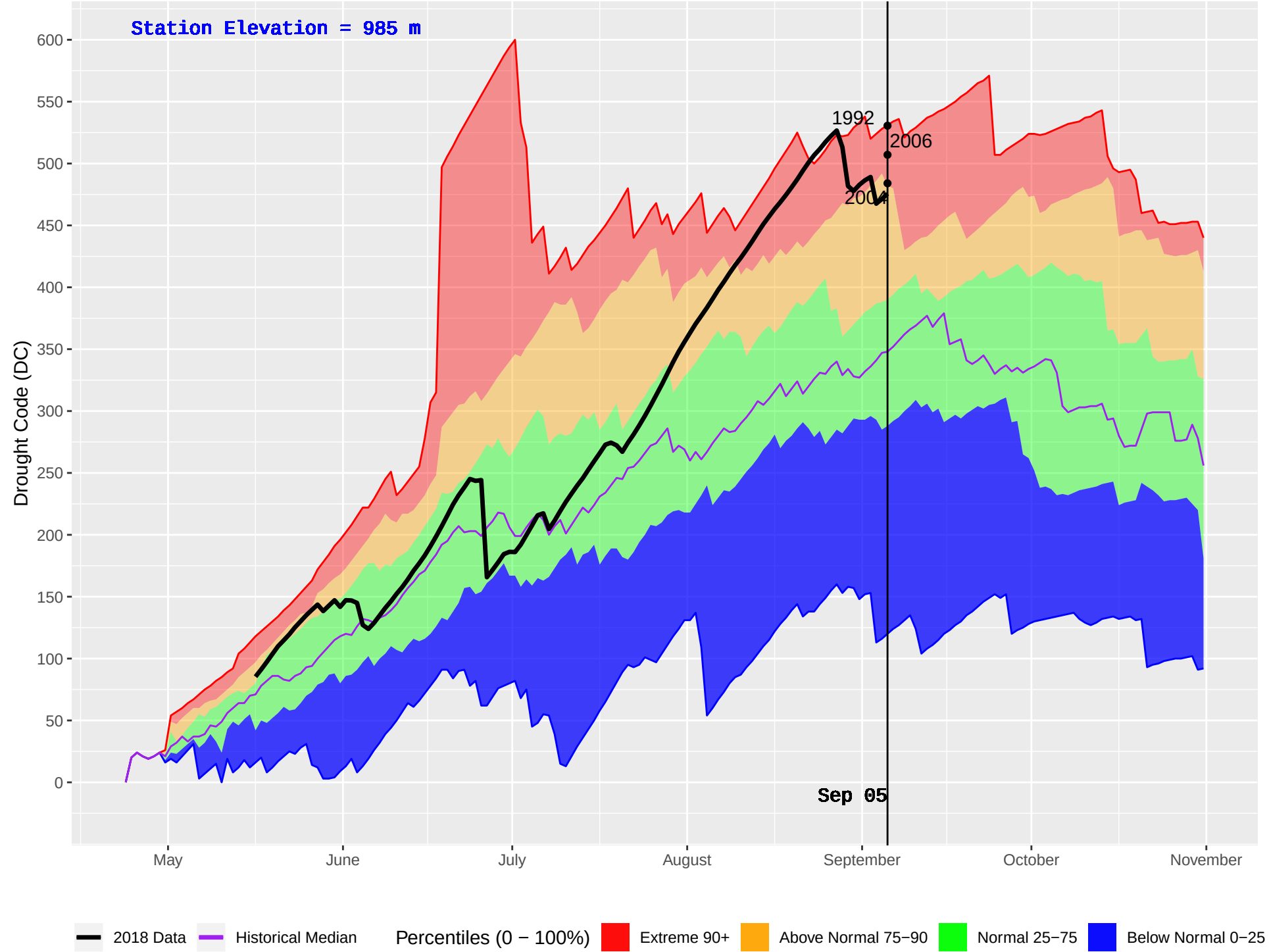
SIFTON (152) : Historical (1988–2016) and Current (2018) Daily Drought Code (DC)
